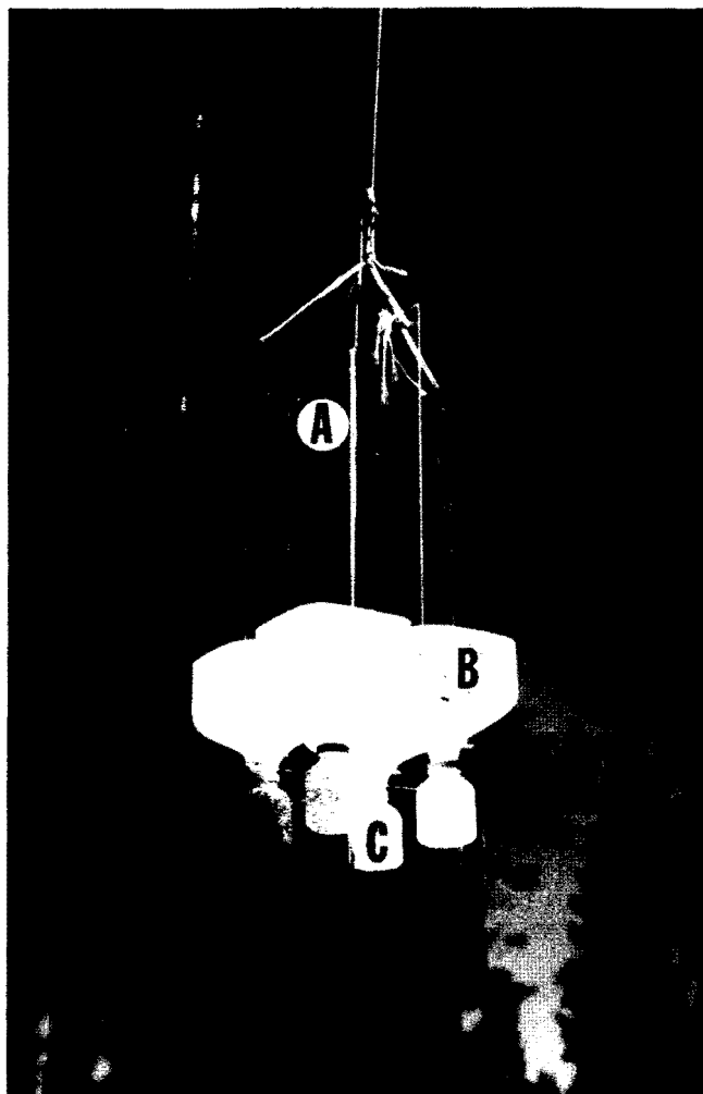
Figure 1.—Omnidirectional passive barrier trap consisting of (A) two Plexiglas panels positioned at right angles; (B) four funnellike collectors bolted to the base of the panels; (C) four plastic bottles to contain trapped insects.
